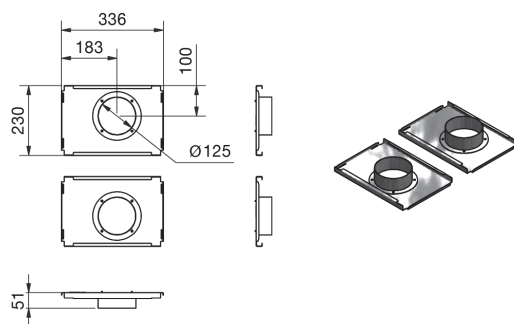
Zehnder ComfoAir 200
